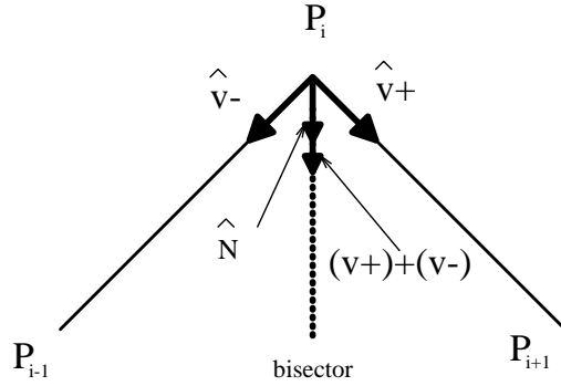
Figure 7: The vectors \hat{v}_- and \hat{v}_+ are defined by the vertices: P_{i-1} , P_i and P_{i+1} . The dashed line indicates the bisector of P_i which coincides with the direction of the vector \hat{v}_- + \hat{v}_+ .
