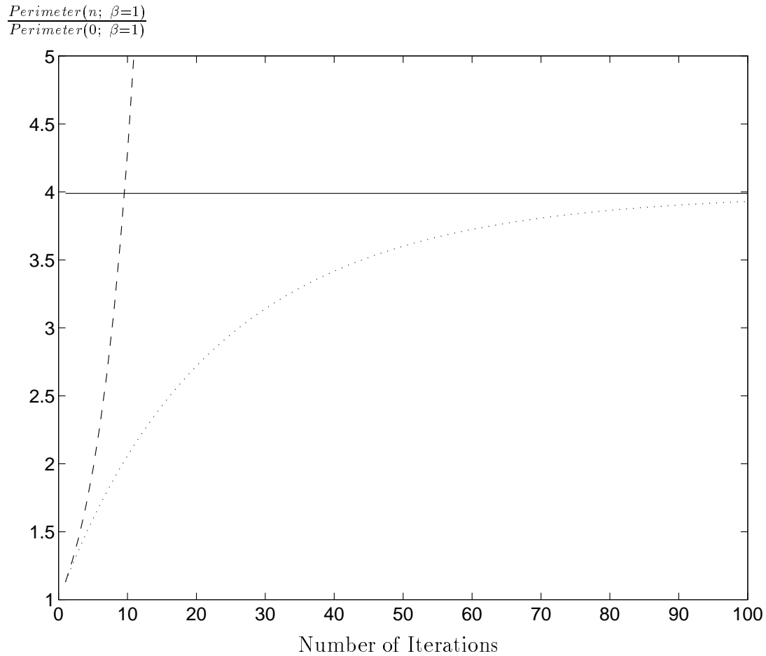
Figure 13: Example of the restrained exaggeration convergence. The ratio between the perimeter of the evolving polygon and the initial one is shown as a function of the number of iterations. The horizontal line is the perimeter of the steady-state polygon. Using the restrained evolution (dotted), the polygon asymptotically reaches the steady state perimeter. On the other hand, the unrestrained evolution (dashed) causes the polygon to ‘explode’.
