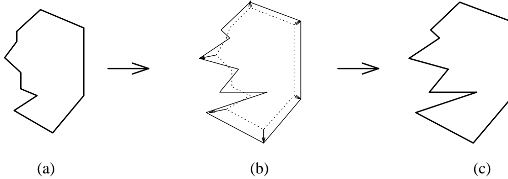
Figure 6: Polygon exaggeration. For each vertex of the initial polygon (a), the normal \hat{N}_i^{(n)} and curvature \kappa_i^{(n)} are calculated. Then, (b) each vertex is moved in the direction of \hat{N}_i^{(n)} by a step proportional to \kappa_i^{(n)} thus creating a caricature effect (c).
