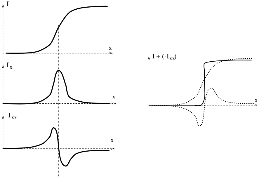
Figure 1: Deblurring a step function, the 1D case.
