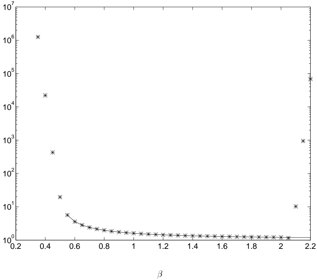
Figure 14: Restrained exaggeration convergence for different bounding forces. The ratio between the perimeter of the evolving polygon and the initial one is given for different values of B = \beta I . The ‘star’ line is a result of 1,000 iterations with the restrained evolution law. The other line is the steady-state result. In the convergence range, 2\alpha < \beta < 2 , ( \alpha = 0.25 ), the two are identical. Outside the convergence range, the polygon ‘explodes’ to infinite perimeter and does not reach a steady-state.
