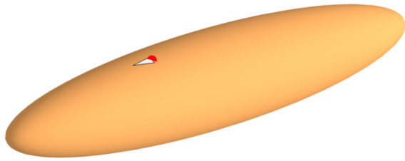
Figure 6: Ellipsoid resulting from compressing a sphere. Arrow shows the direction in which a KVF is searched for.
