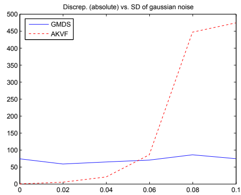
Figure 4: Quality vs. Standard Deviation (absolute discrepancy)
