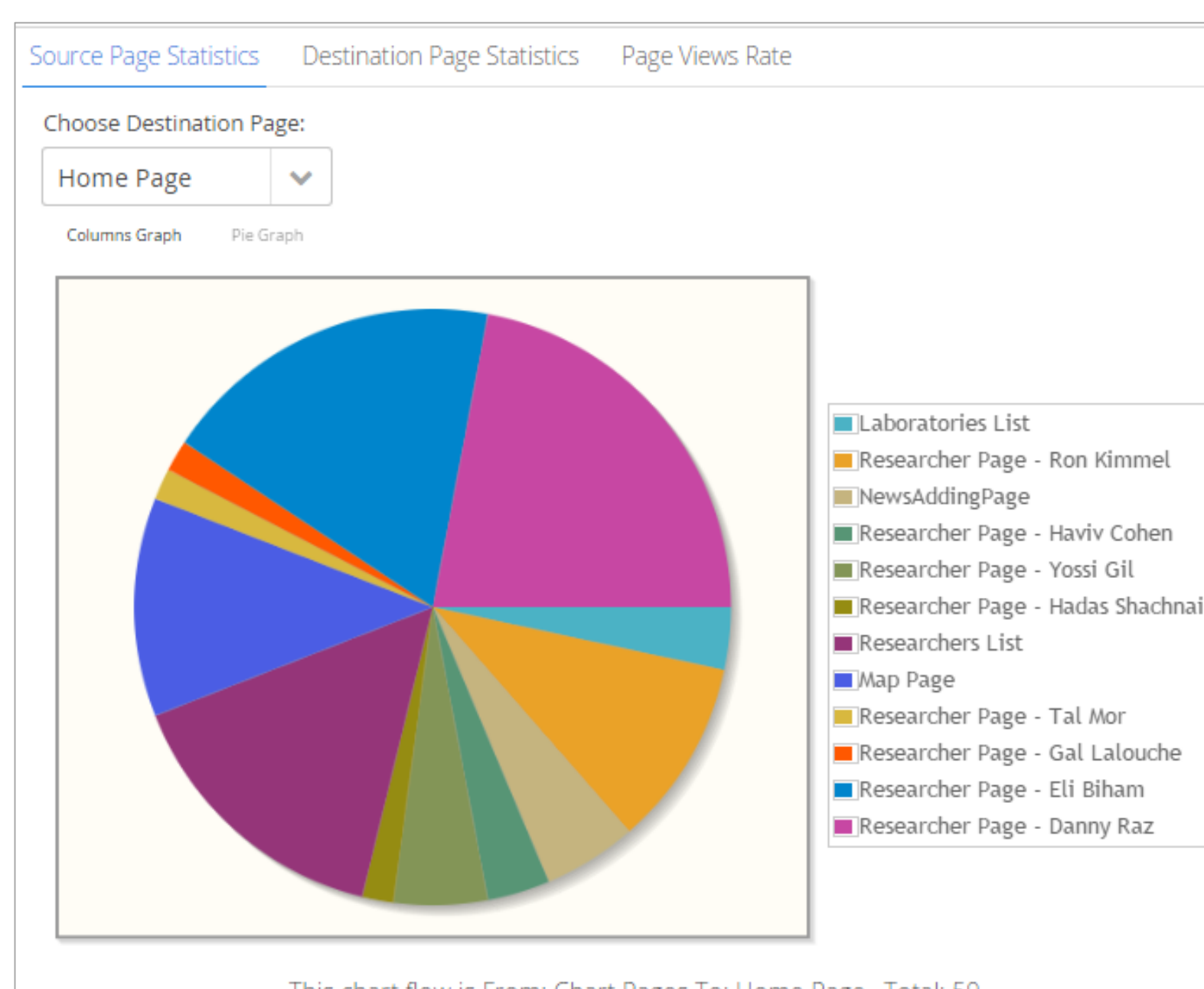
Statistics
