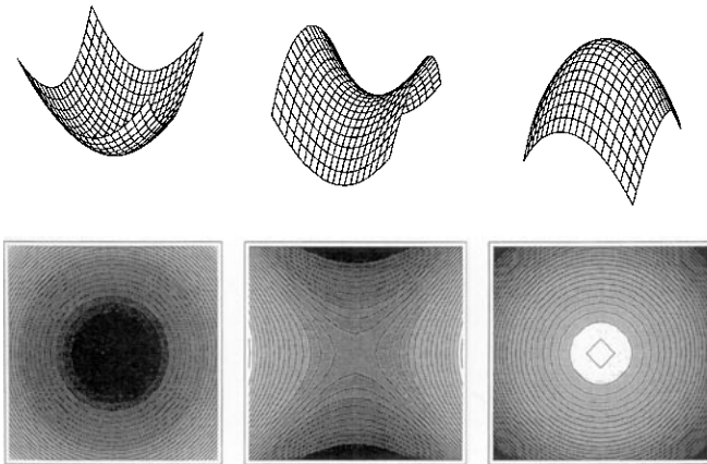
FIG. 2. The three types of singular points that characterize the Morse function are the minimum, the saddle, and the maximum points. The lower frames display the equal height contours painted on a gray-level image that represents the heights.
