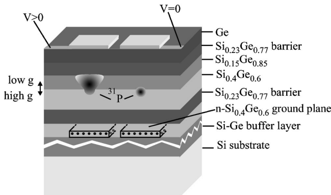
FIG. 5. The left transistor gate is biased V > 0 , producing single-qubit unitary transformations in the left SRT. The right gate is unbiased: V = 0 . The n\text{-Si}_{0.4}\text{Ge}_{0.6} ground plane is counterelectrode to the gate, and it also acts as FET channel for sensing the spin.
