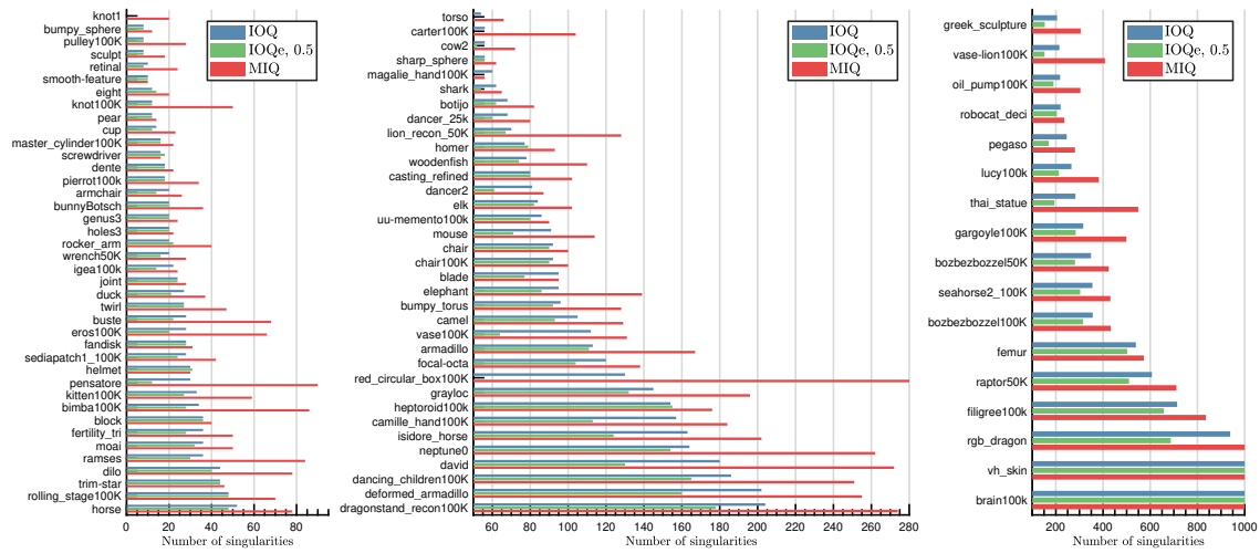
Fig. 1. Number of singularities.
