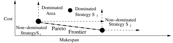
Figure 2: A Pareto frontier. Strategies S_1 and S_2 form the Pareto frontier. S_1 dominates S_3 .
