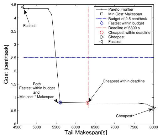
Figure 7: Pareto frontier and examples of best points for various user utility functions. Input: Experiment 11 (Table V).
