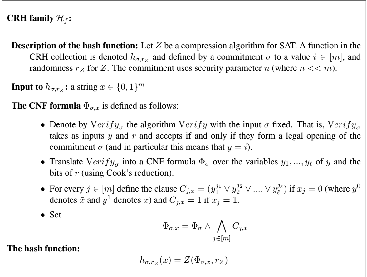
Figure 1: The construction of Collision Resistant Hash from any one-way function.
