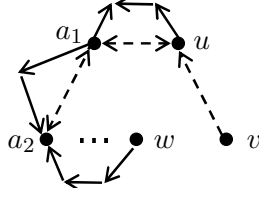
Figure 2: Proof of Lemma 3. Dashed arrows represent white edges, while solid arrows represent black edges. If v removes u from B_t(v) by receiving m(u) from w , then there is an undirected black path between u and w .
