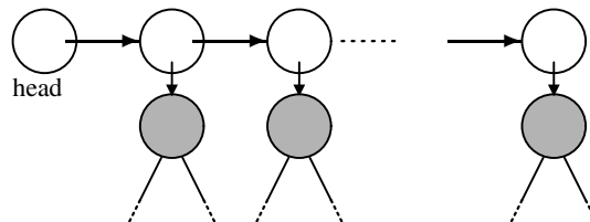
Fig. 1. In this example, the privatizing transaction sets the head to NULL and privatizes the dark items and their subgraphs. Other transactions write to the dark items; each transaction writes to a different one.
