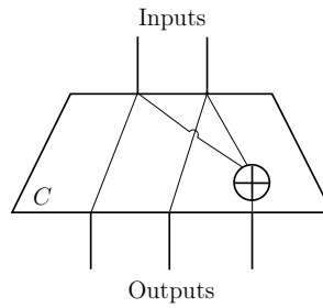
Fig. 2. A 2-universal circuit
