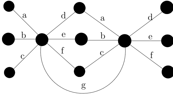
Figure 1: Rainbow diameter is not monotone
