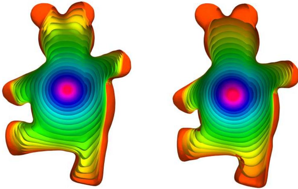
Figure 4.2: \epsilon_2 effectiveness demonstrated on a teddy mesh foliation result. (left) \epsilon_2 = 6e-7 . (right) \epsilon_2 = 6e-5 .
