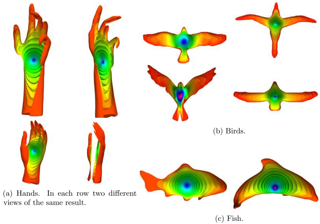
Figure 5.6: Closely related meshes, with the singular point being located in similar positions along the meshes.
