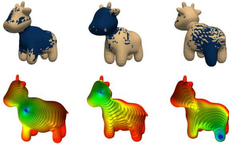
Figure 5.2: Conformal distortion for 3 different results obtained using the same input mesh, and different injection point positions. The distortion is measured between the input mesh and the innermost layer. (top) The input mesh colored by the conformal distortion values, dark-blue faces are faces with distortion value smaller than 1.5. (bottom) The corresponding foliations of the input domain, the injection point is in the center of the innermost layer.
