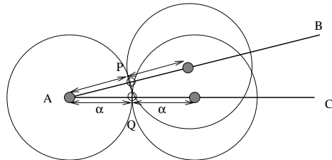
Fig. 3. The unweighted subdividing alpha cannot exist when \angle A < 2 \arcsin(\frac{1}{4}) . There must exist a ball centered on A . Also, there must be some balls centered on the segments \overline{AP} and \overline{AQ} . Those balls will inevitably intersect and create an extra edge in the alpha complex.
