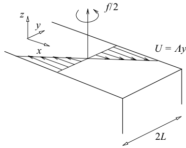
FIGURE 1. Schematic of the Couette flow, with velocity (Ay, 0, 0) , of a three-dimensional Boussinesq fluid with constant Brunt–Väisälä frequency N . The domain rotates around the (vertical) z -axis at rate f/2 ; it is unbounded in the x - and z -directions, and bounded in the y -direction by two rigid walls separated by a distance 2L .
