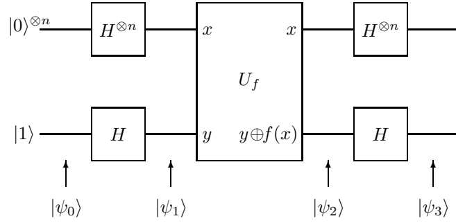
Fig. 1. The Deutsch-Jozsa algorithm (which is a quantum subroutine common to Simon, Grover, Bernstein-Vazirani and other algorithms)
