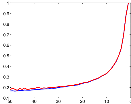
Fig. 2. As the number of robots increases (represented as the X axes), the ratio between the performance of the simple robots and the upgraded robots decreases. For groups of over 30 robots, the upgraded robots achieve an efficiency of approximately 20% than this of the simple robots (namely, 5 times larger an exploration time).
