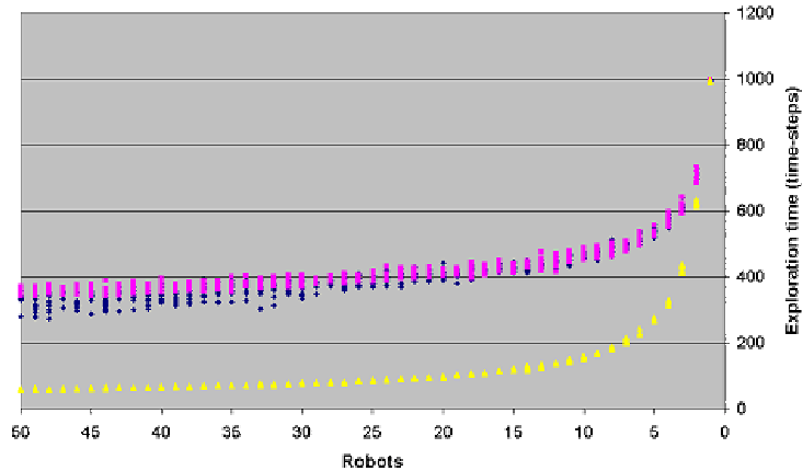
Fig. 1. This chart depicts the range of exploration times of three groups of robots, tested in a variety of random graphs. The lower curve represents the exploration time of the original group, comprising “basic robots”, to whom the exploration algorithm used was originally designed. The upper curves represents the exploration time of the “upgraded robots”.
